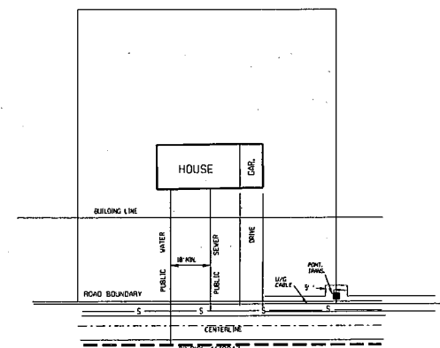
TYPICAL LOT LAYOUT (NOT TO SCALE)
