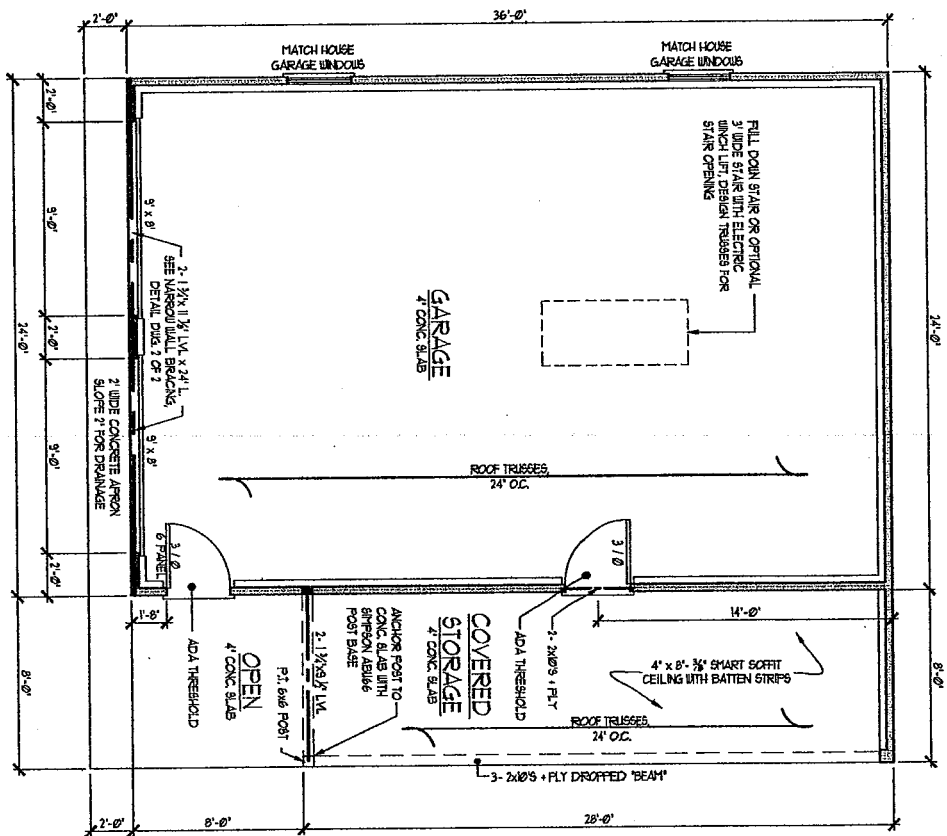
PLAN 1/4" = 1' - 0"
