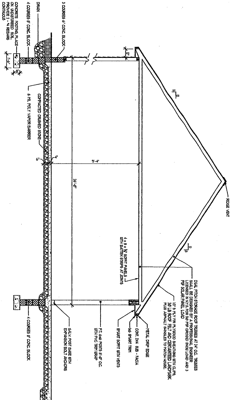
TYPICAL WALL SECTION AT COVERED STORAGE 3 / 8" = 1' - 0"
